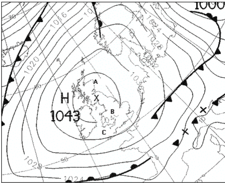
Anticyclone
