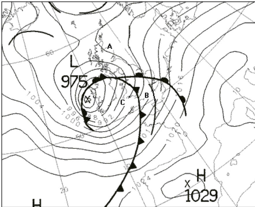
Depression
